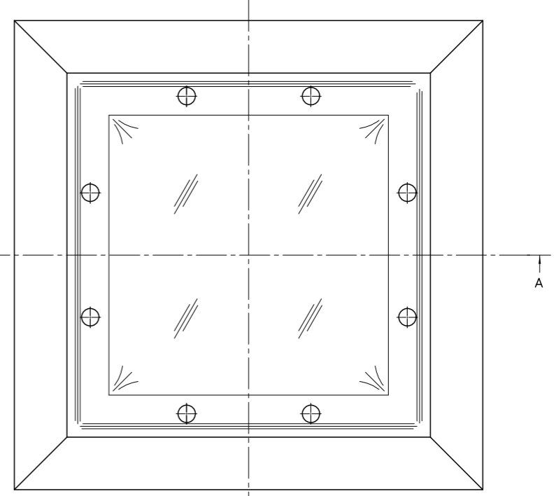
PLAN Scale 1/4
