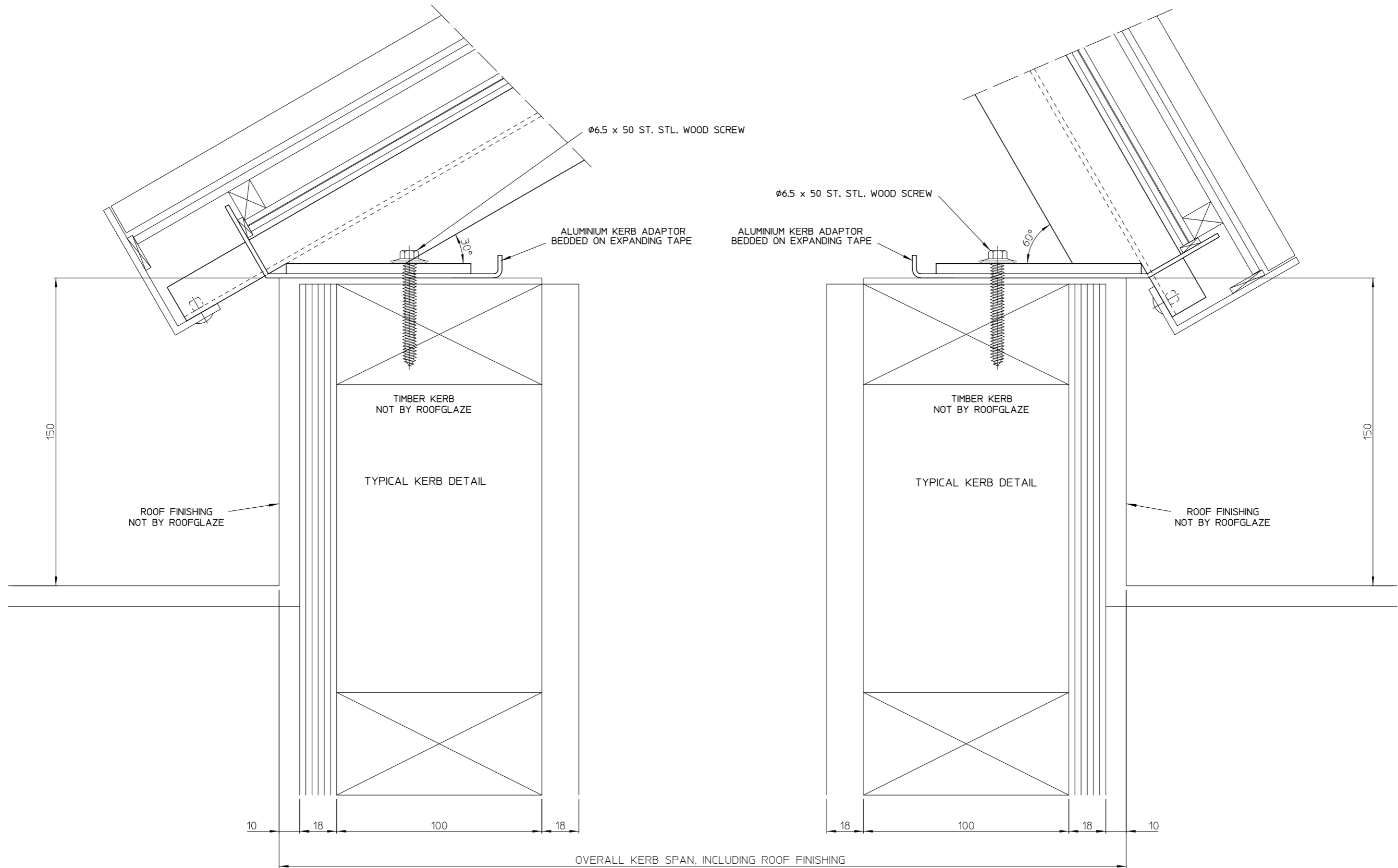
SECTION C-C
