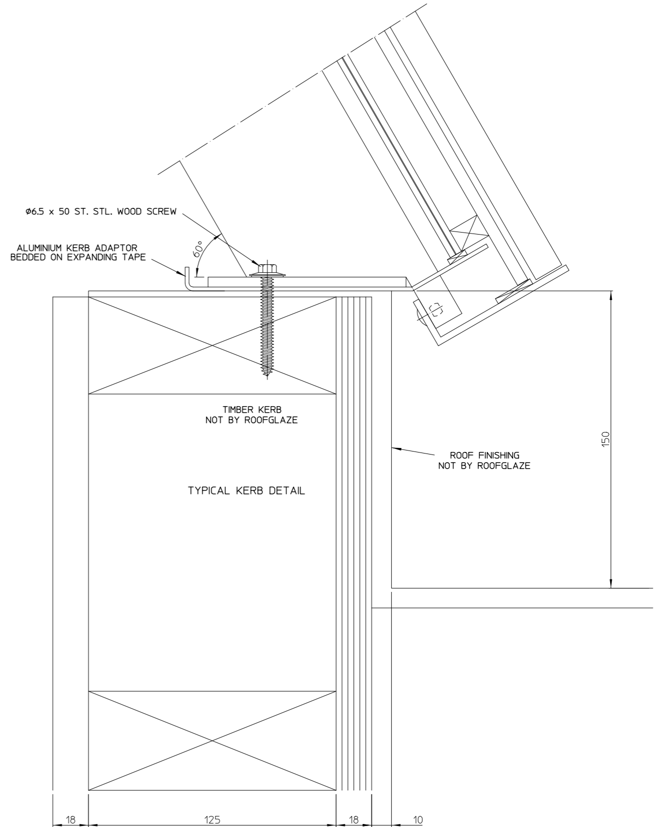
SECTION C-C
