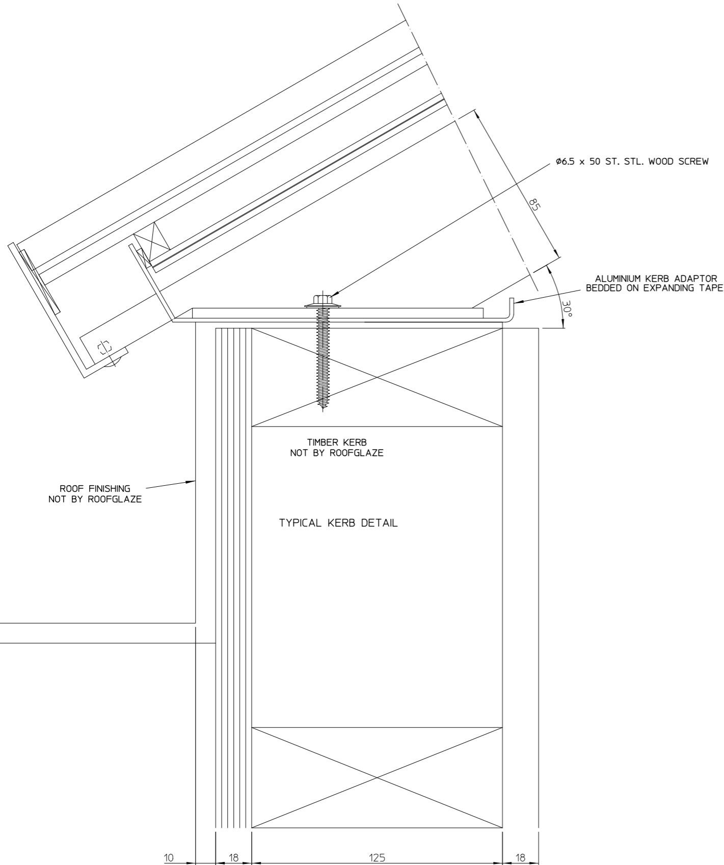
SECTION B-B
