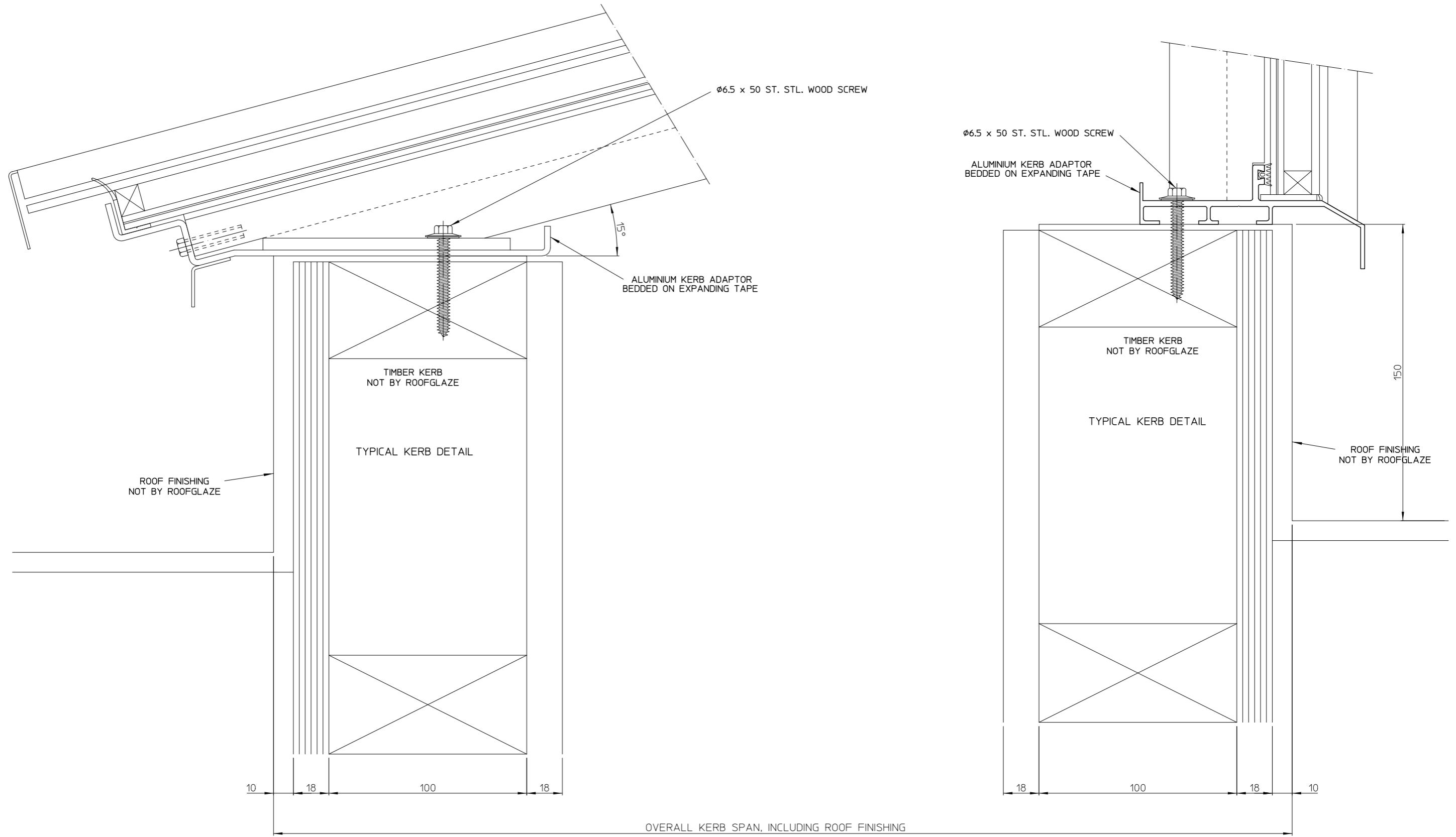
SECTION C-C
