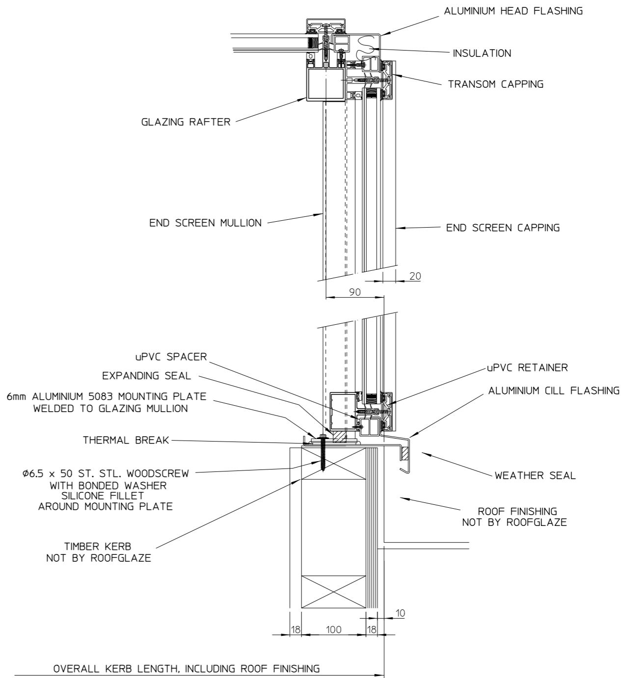
SECTION E-E
