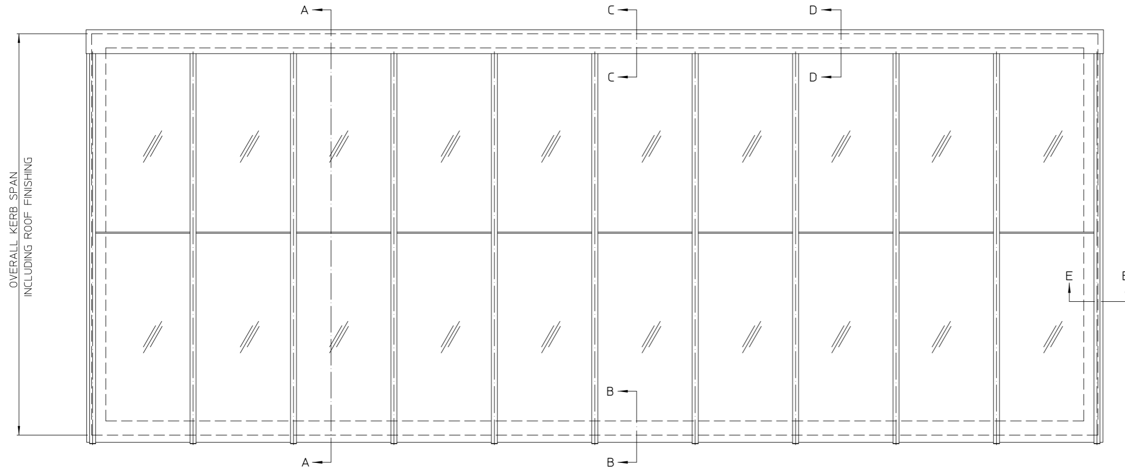
PLAN VIEW
