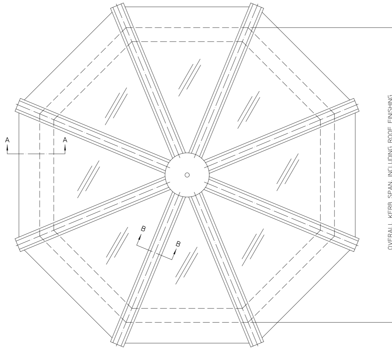
PLAN VIEW
