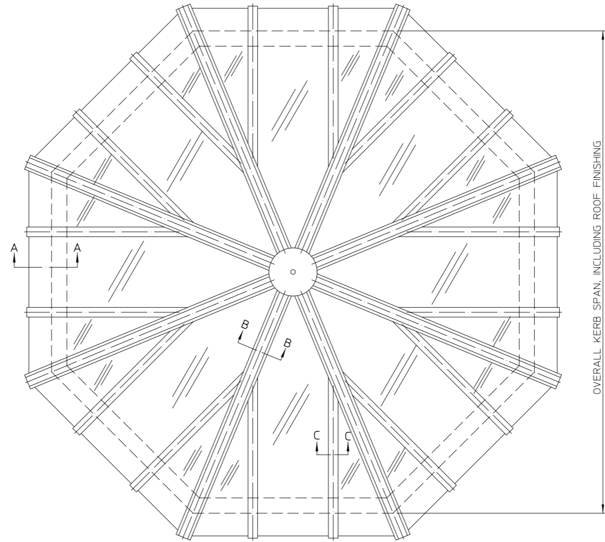
PLAN VIEW
