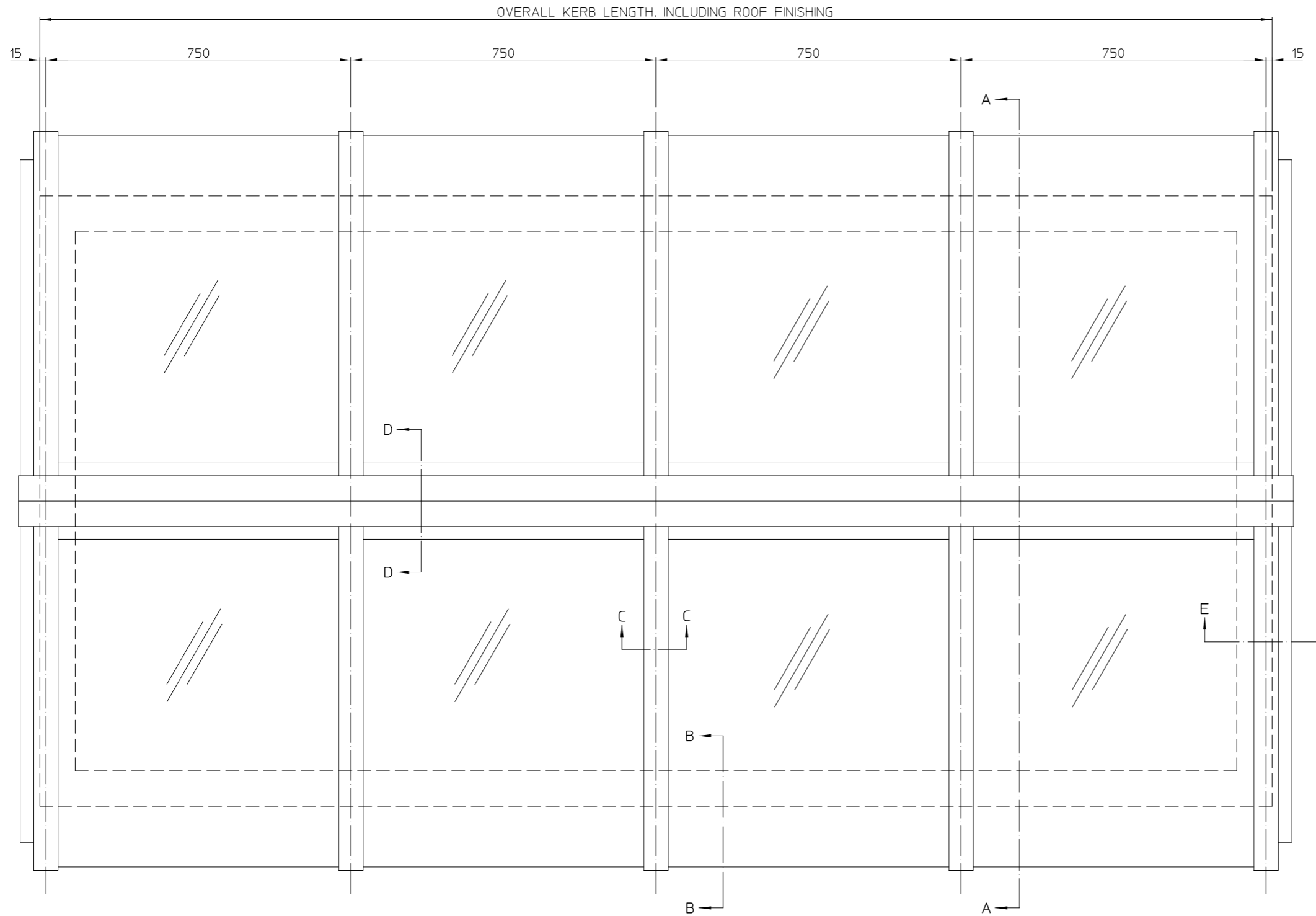
PLAN VIEW
