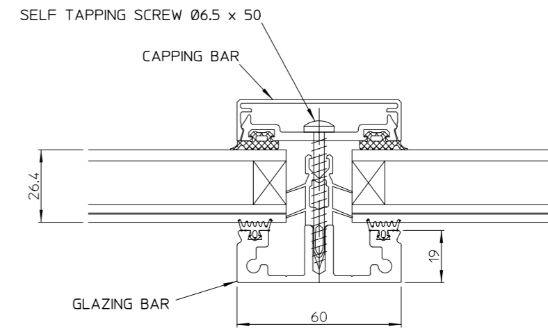
SECTION C-C RAFTER SECTION VIEW
