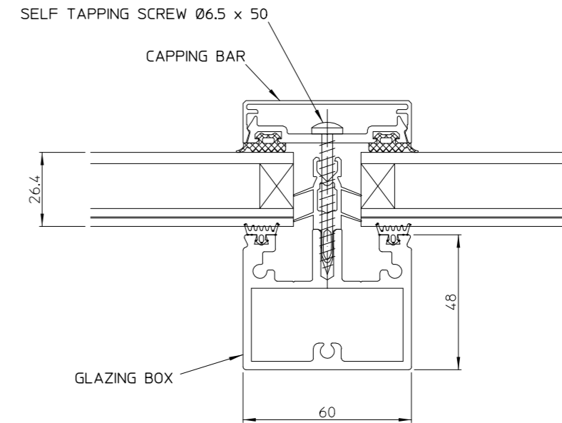
SECTION C-C RAFTER SECTION VIEW
