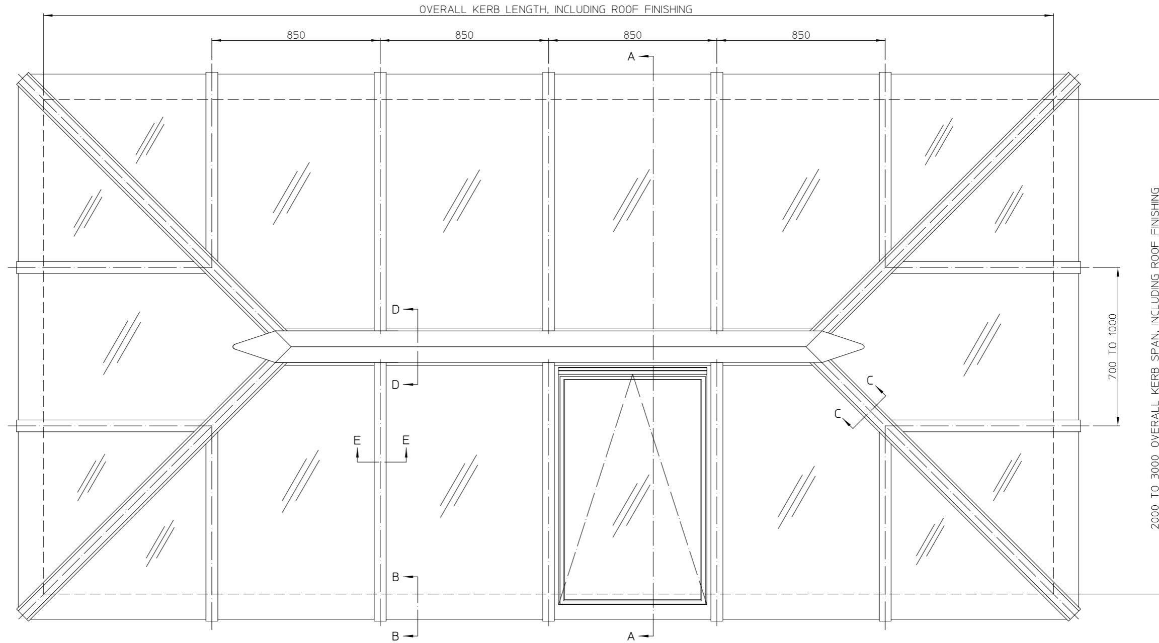
PLAN VIEW
