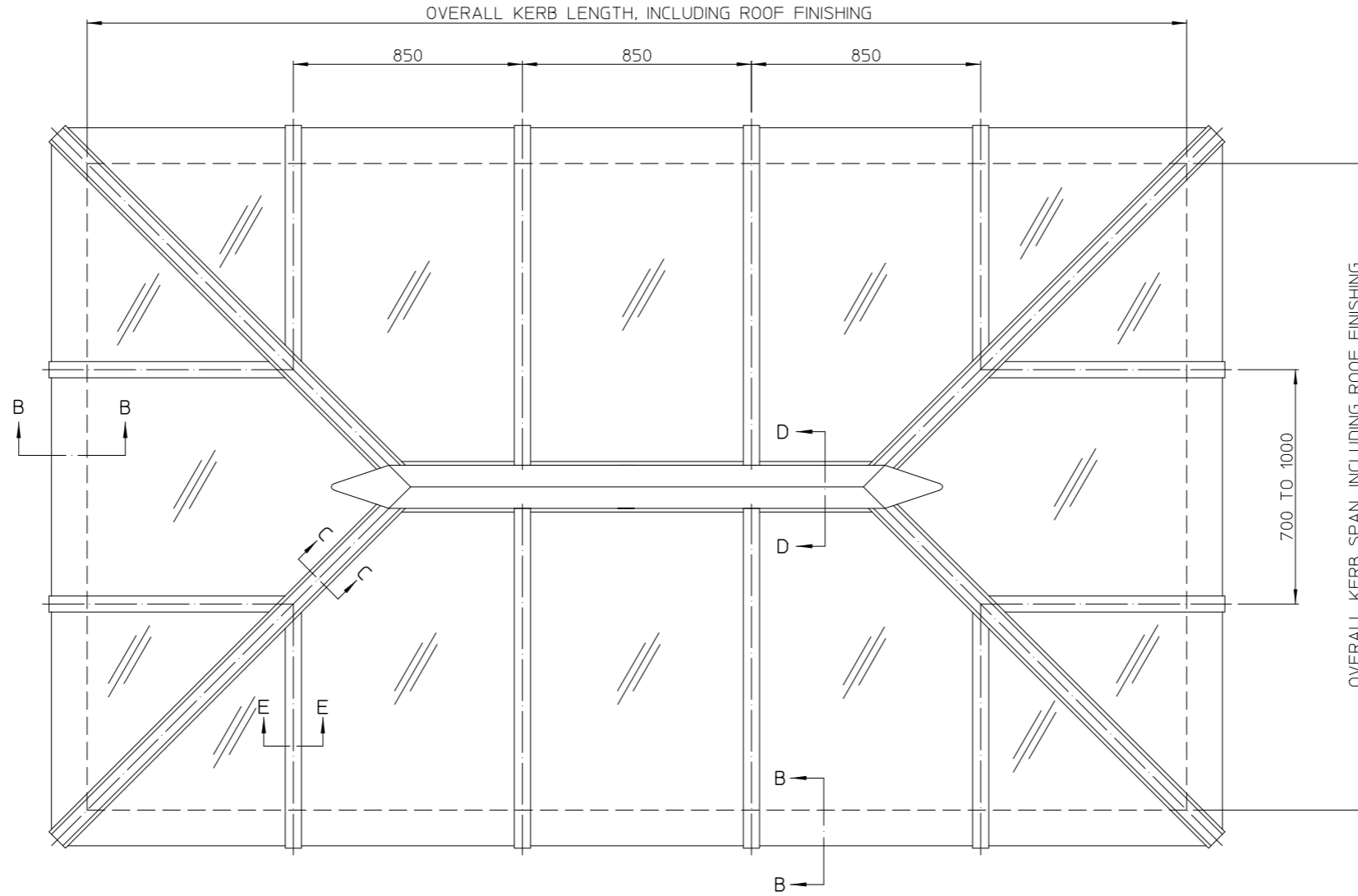
PLAN VIEW
