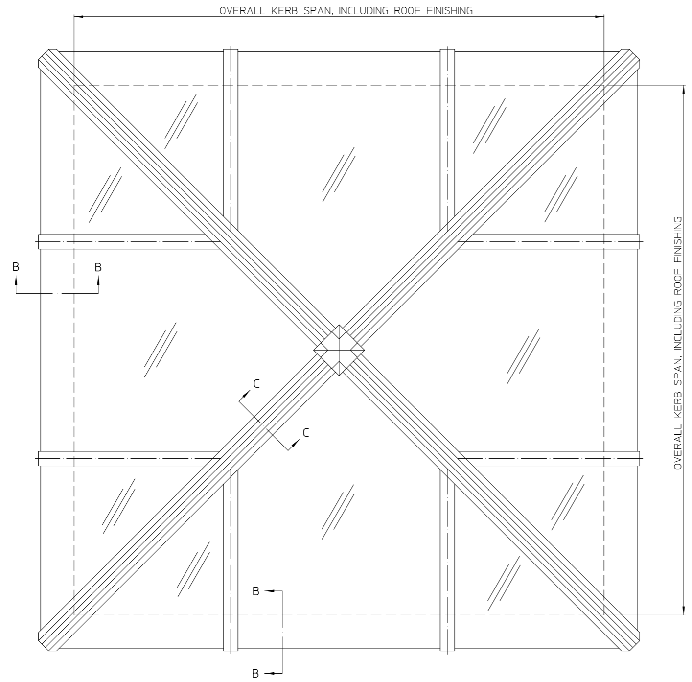
PLAN VIEW
