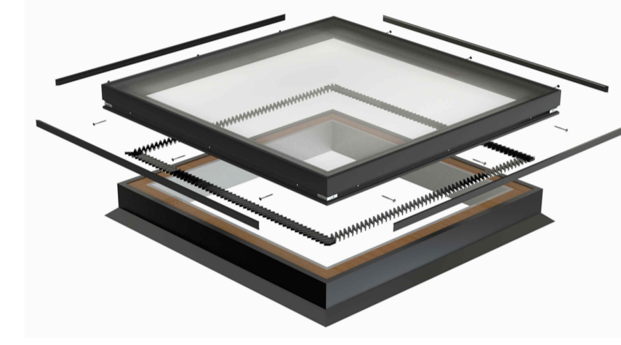
EXPLODED INSTALL GUIDE
