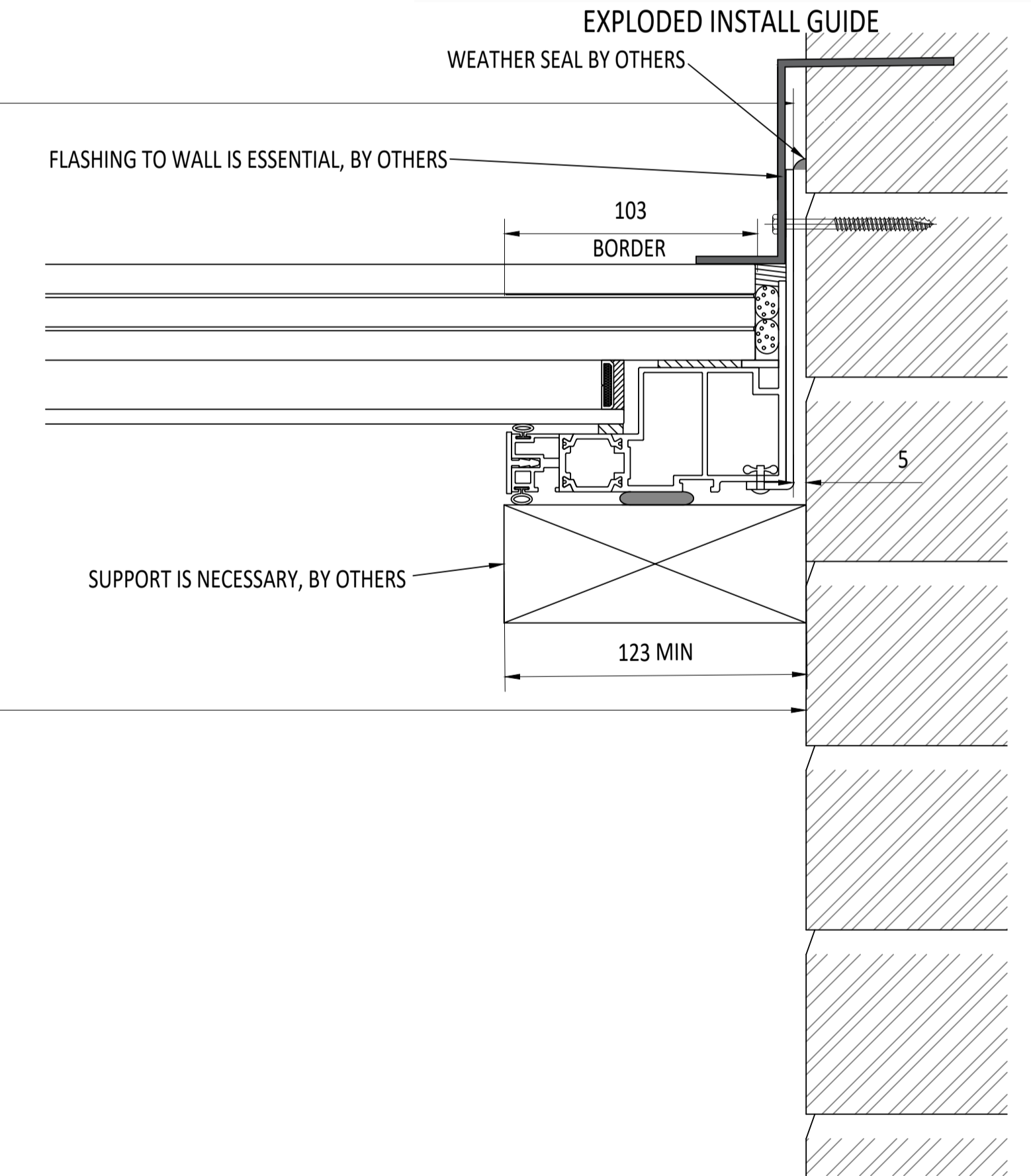
SECTION B-B
