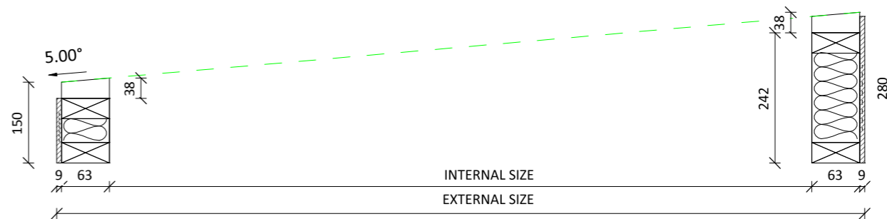
2 Section 1 Scale @ 1:10
