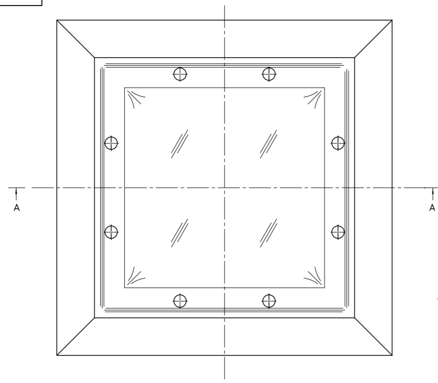
PLAN Scale 1/4
