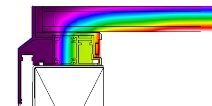
THERMAL IMAGING OF FRAME
