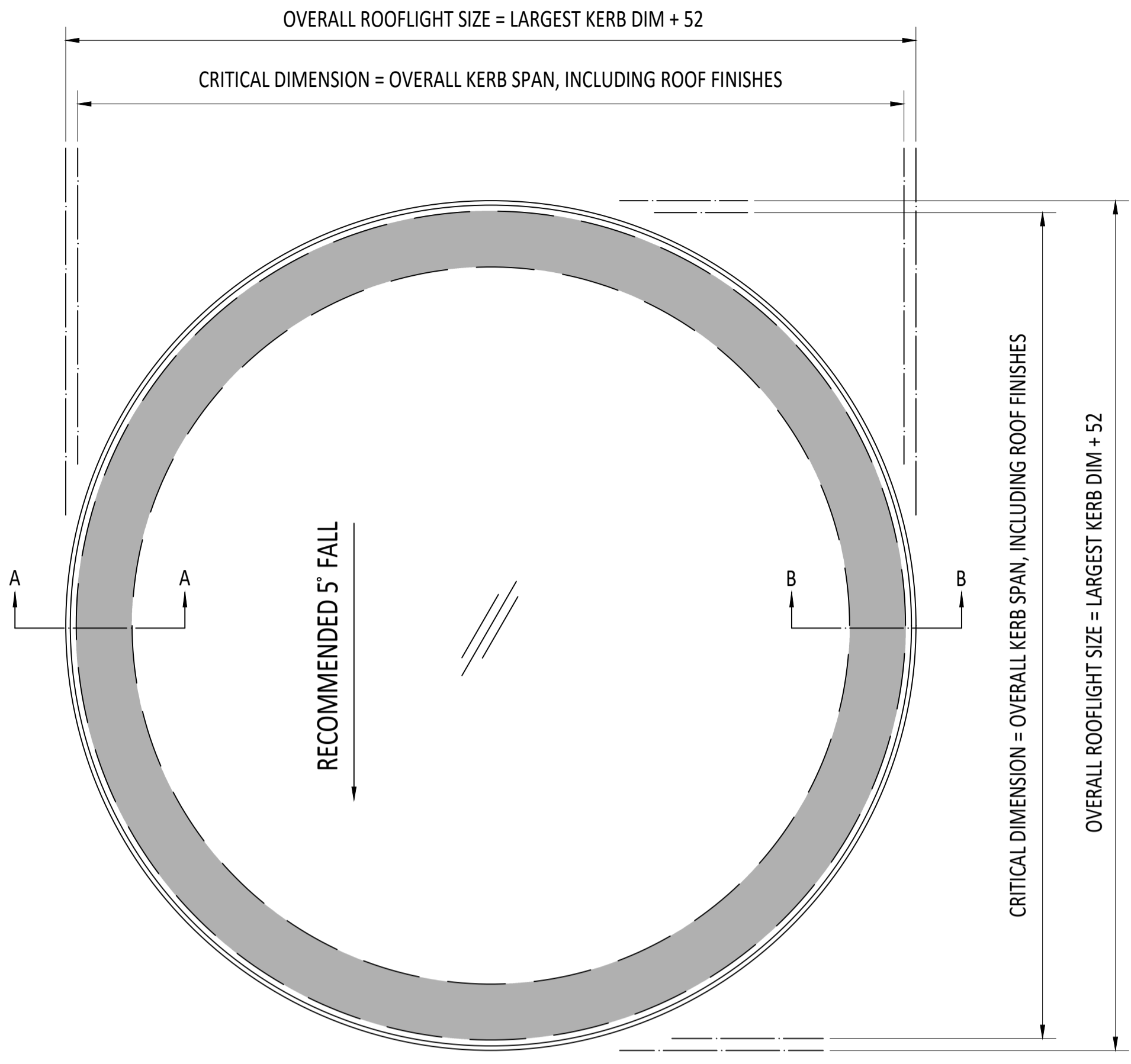
PLAN VIEW True view on slope
