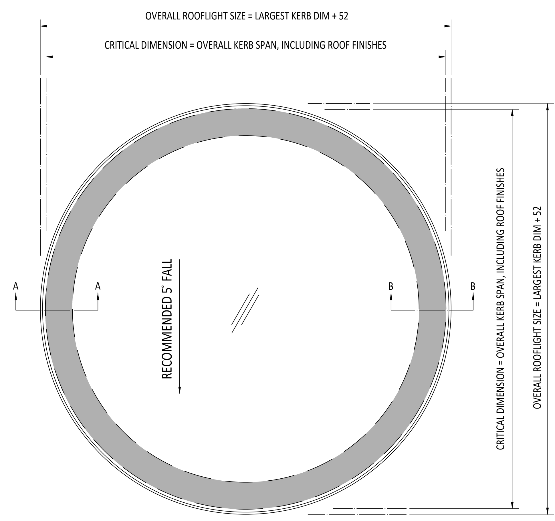
PLAN VIEW True view on slope
