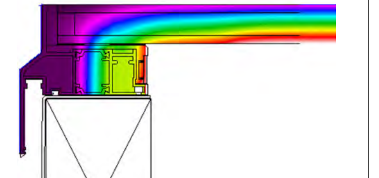
THERMAL IMAGING OF FRAME
