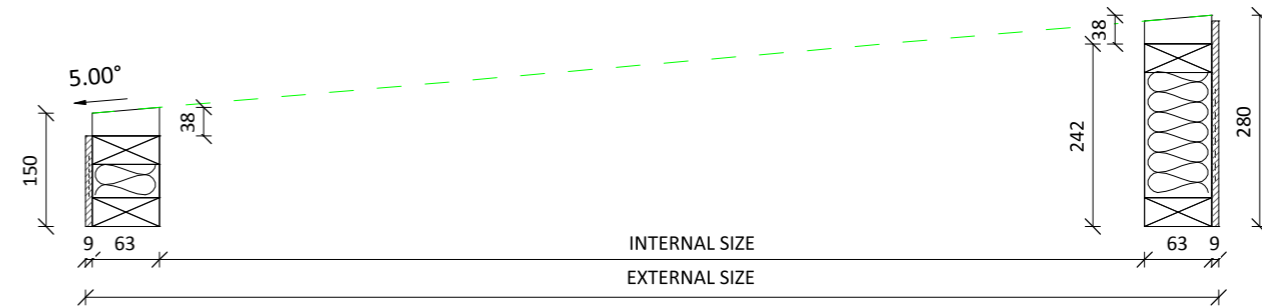
2 Section 1 Scale @ 1:10
